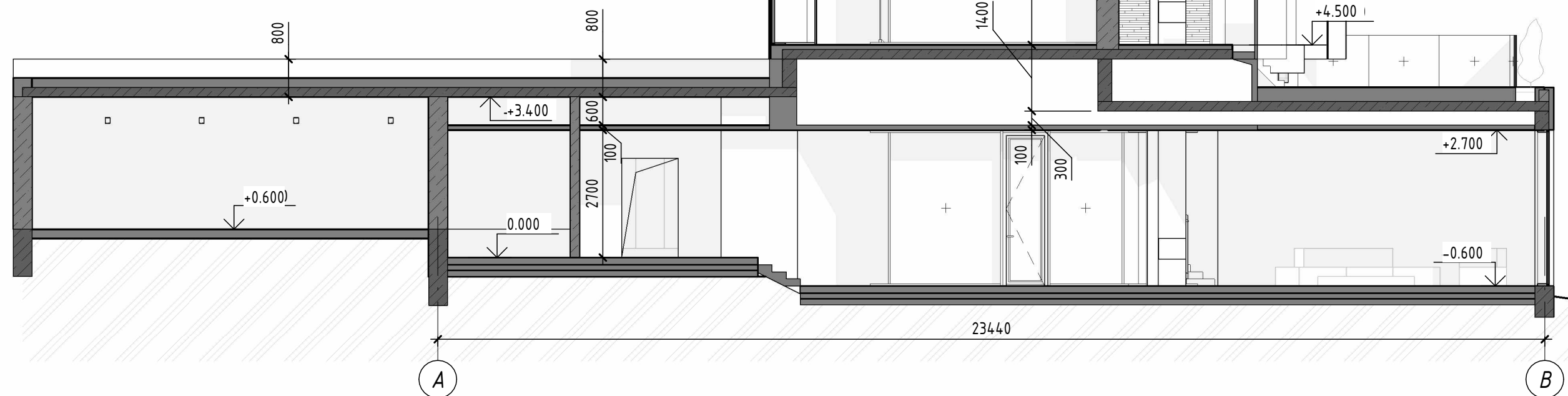
Section 2-2
