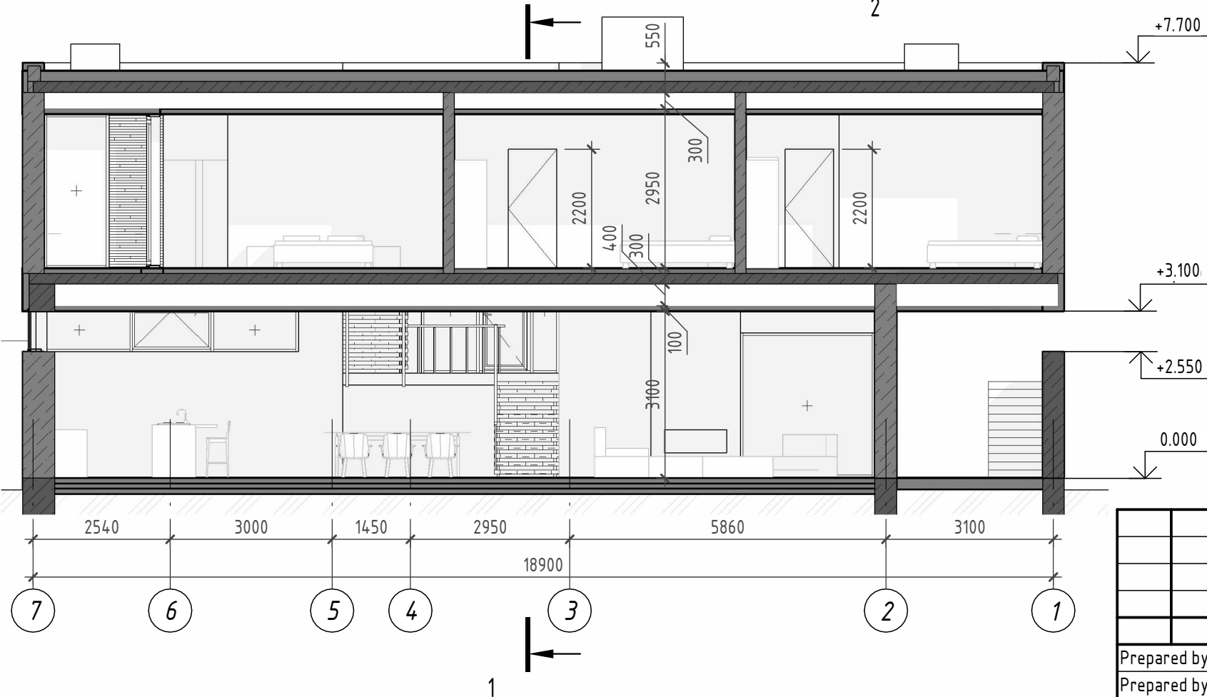
Section 2-2
